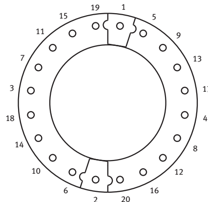
20 - HOLE RING
